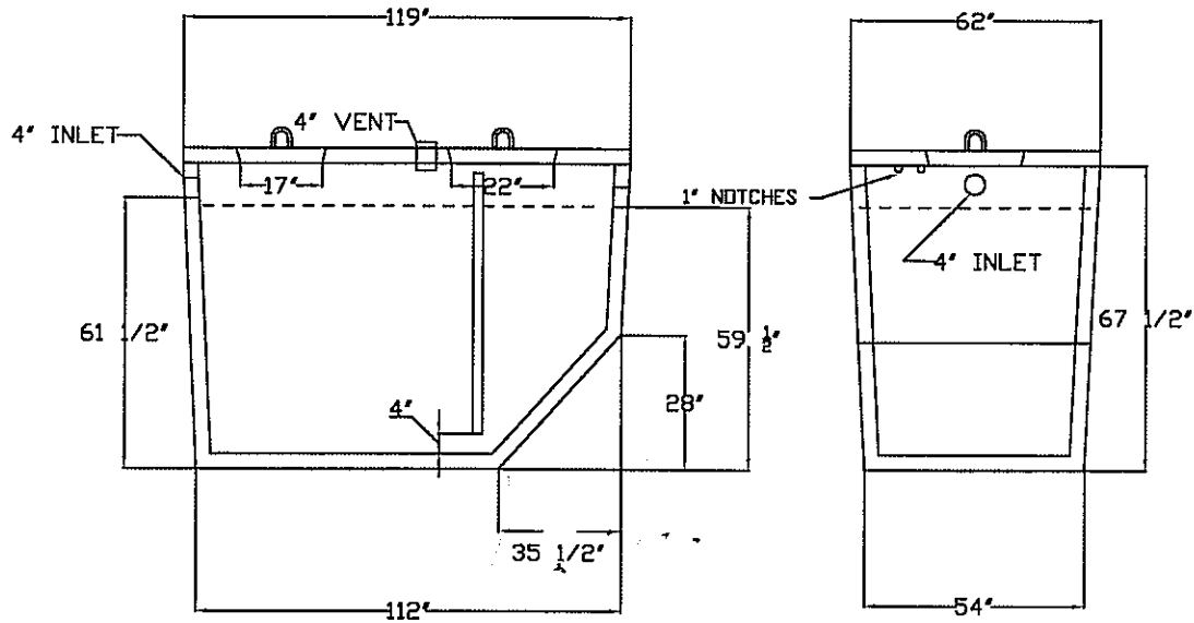
SIDE VIEW
