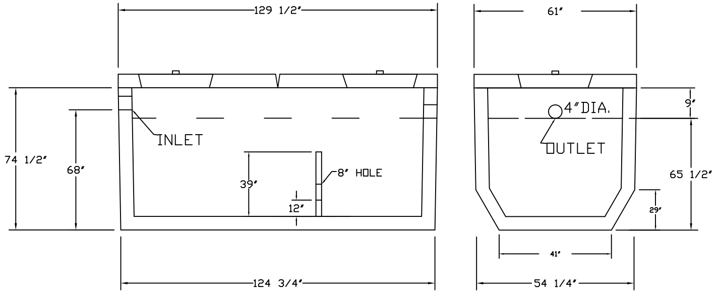
SIDE VIEW
