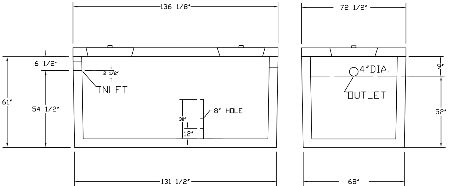
SIDE VIEW
