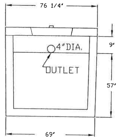
END VIEW
