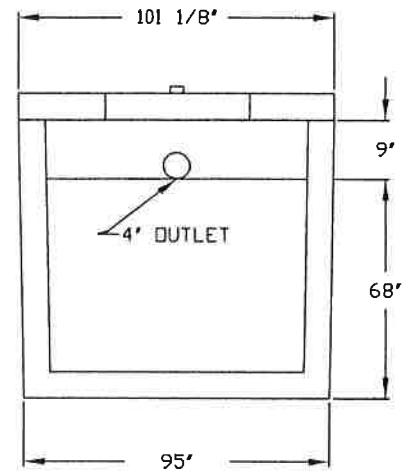
END VIEW
