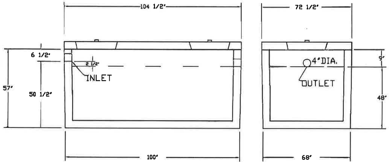
SIDE VIEW
