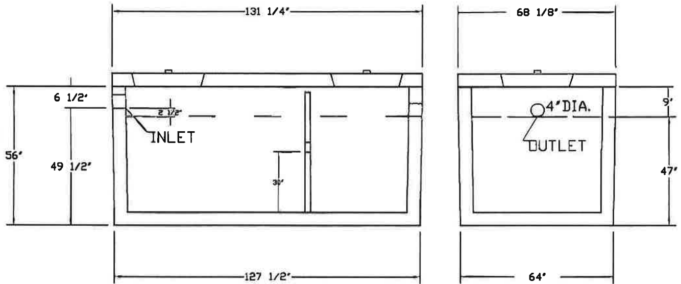
SIDE VIEW
