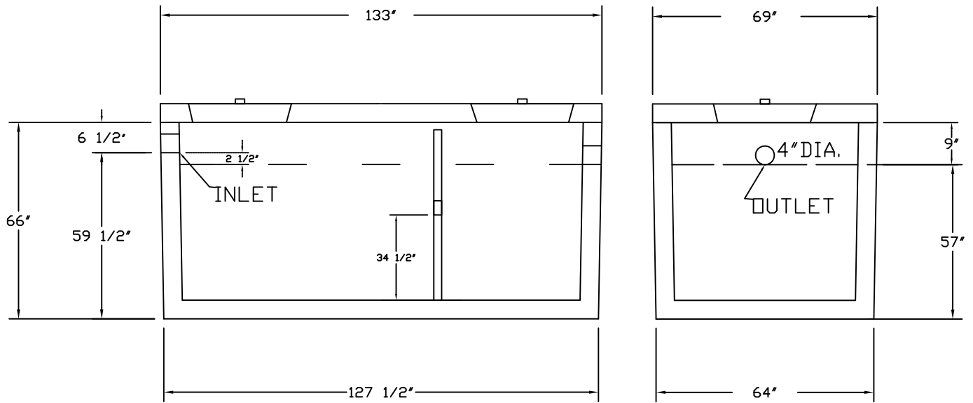
SIDE VIEW
