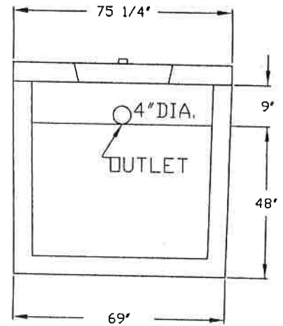
END VIEW
