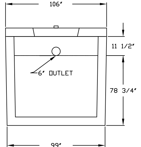
END VIEW
